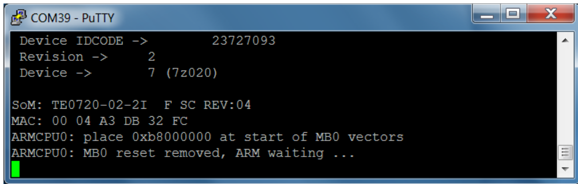
Figure 18: Debug demo t01_l. Execution of the ./t01_s.elf example from the SD card.
