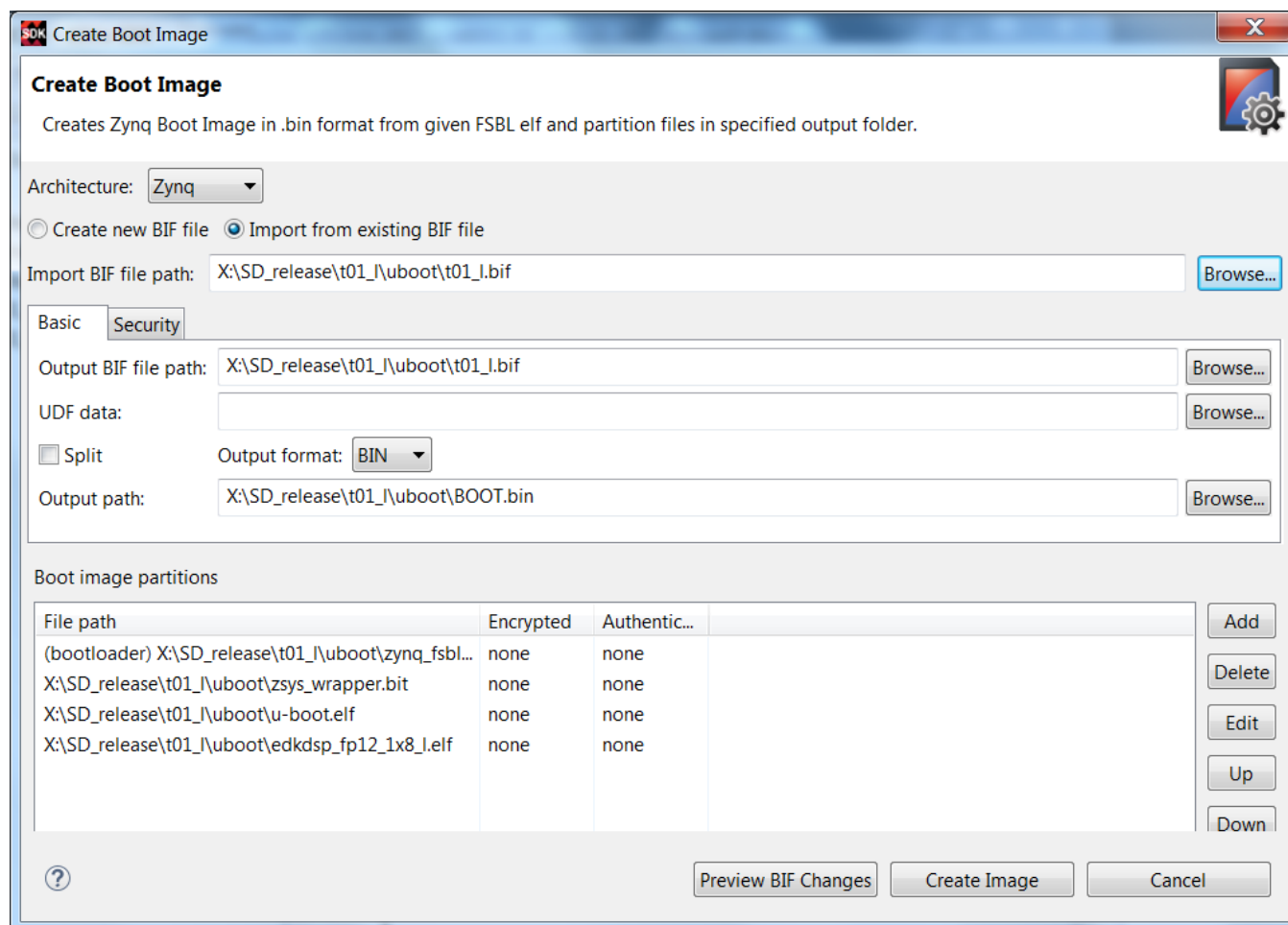
Figure 28: Create BOOT.bin for the t01_l demo.
