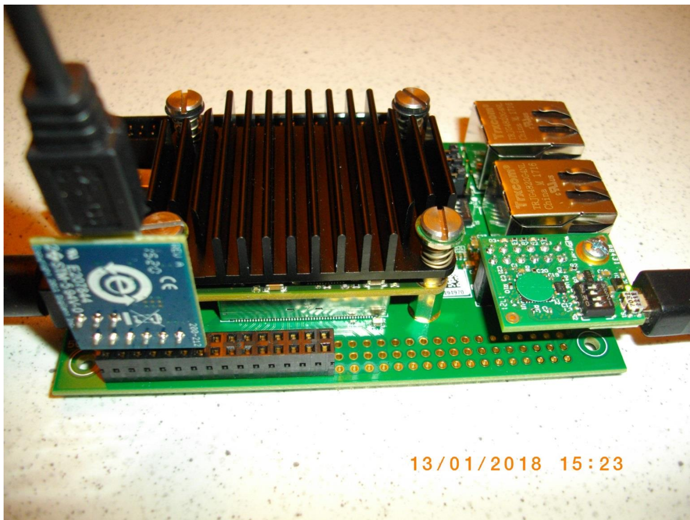
Figure 5: MicroUSB cable: Pmod USBUART. MiniUSB cable: XMOD FTDI JTAG adapter.
